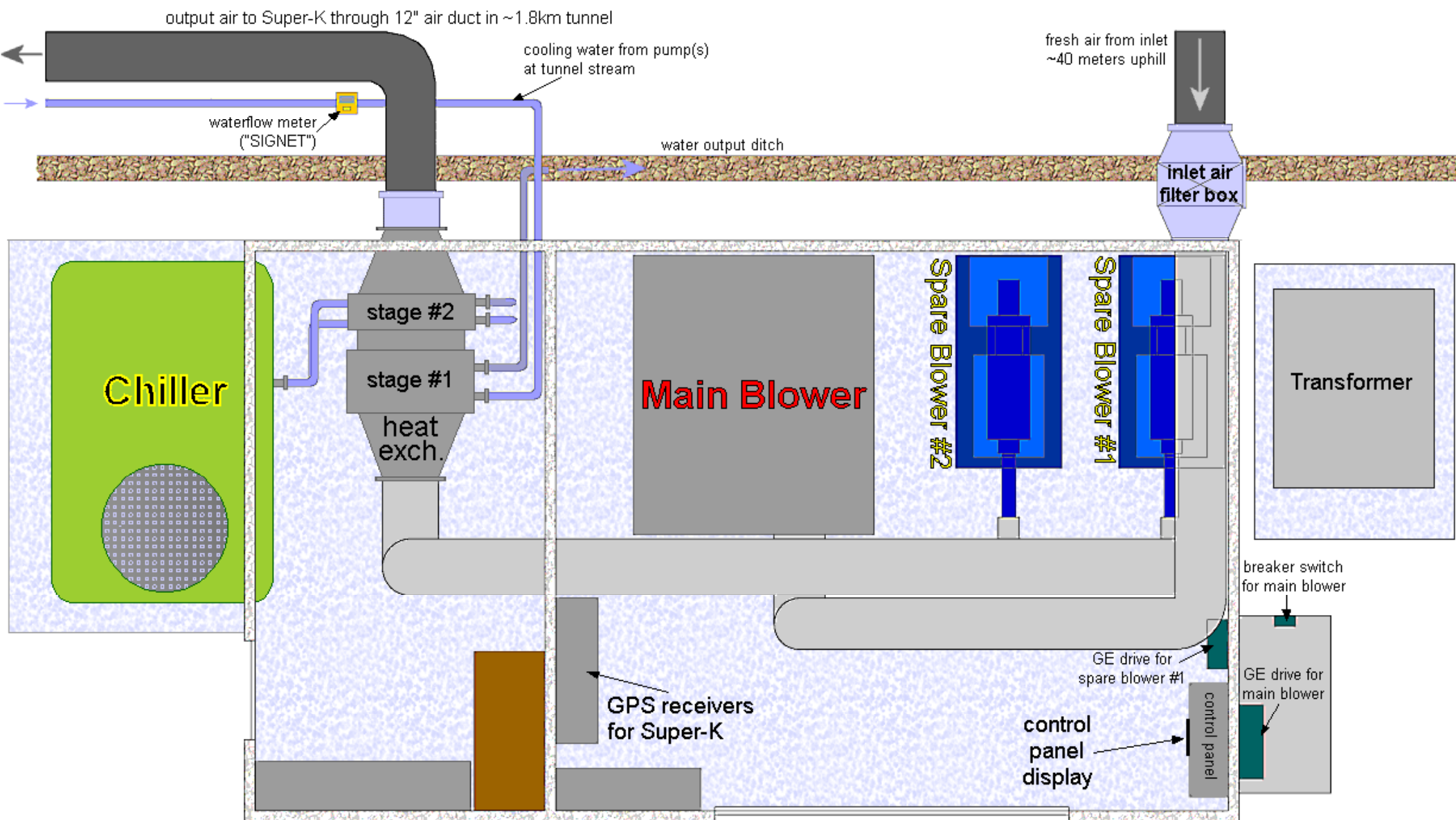
Radon Hut System Layout
