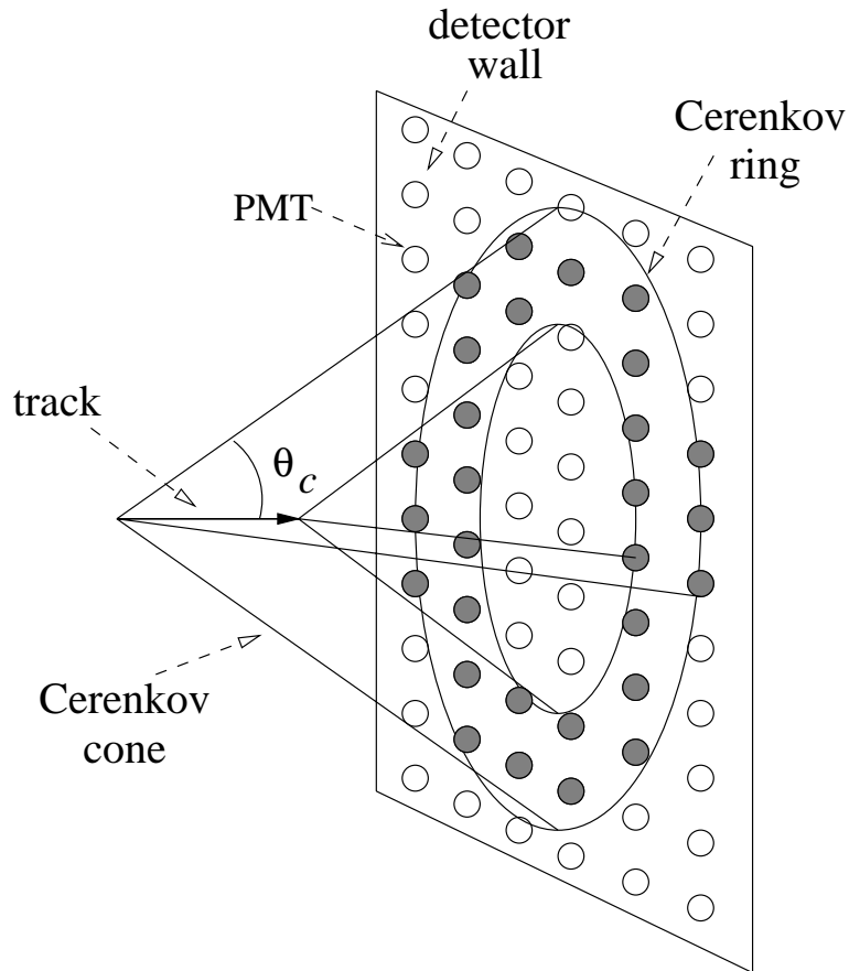
Figure 3.1: Čerenkov geometry
