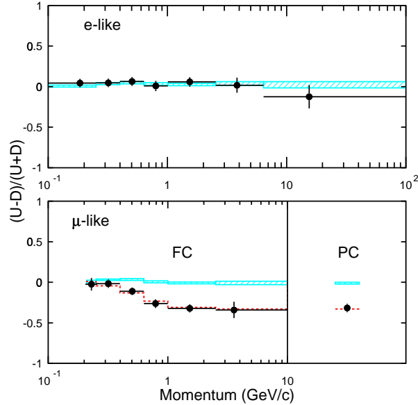
Fig. 3. Up-down asymmetry as a function of momentum for e -like and \mu -like events. The boxes display no-oscillation prediction, while the solid lines result from the \nu_\mu \leftrightarrow \nu_\tau oscillations with the best-fit parameters.
