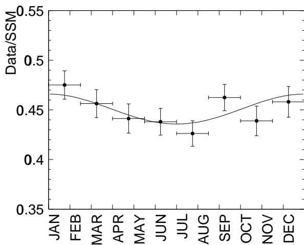
FIG. 4: Seasonal variation of the solar neutrino flux. The curve shows the expected seasonal variation of the flux introduced by the eccentricity of the Earth's orbit. Error bars show statistical errors only.
