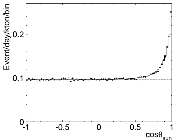
FIG. 1: \cos\theta_{\text{sun}} distribution for reconstructed energy E = 5.0\text{--}20.0 MeV. The points represent observed data, the histogram shows the best-fit signal level plus background, and the nearly horizontal line shows the estimated background. The peak at \cos\theta_{\text{sun}} = 1 is due to solar neutrinos.
