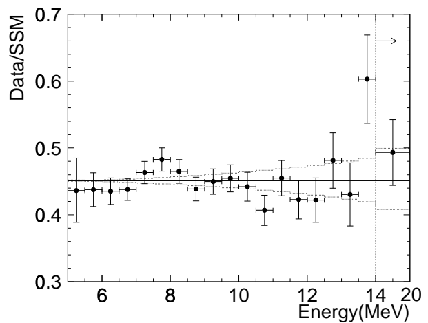
FIG. 3: The measured {}^8\text{B} + \text{hep} solar neutrino spectrum relative to that of Ortiz et al. normalized to BP2000. The data from 14 MeV to 20 MeV are combined into a single bin. The horizontal solid line shows the measured total flux, while the dotted band around this line indicates the energy correlated uncertainty. Error bars show statistical and energy-uncorrelated errors added in quadrature.
