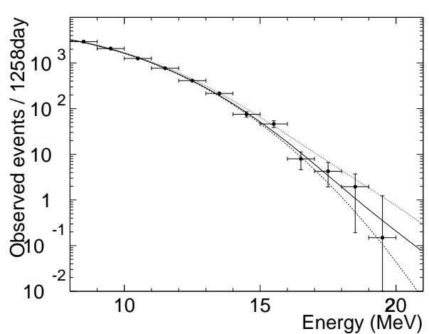
FIG. 5: Energy spectrum of recoil electrons produced by ^8\text{B} and hep neutrinos, in 1 MeV bins. The points show data with statistical error bars. The curves show expected spectra with various hep contributions to the best-fit ^8\text{B} spectrum. The solid, dotted, and dashed curves show the spectrum with 1, 4.3, and 0 times the BP2000 hep flux, respectively.
